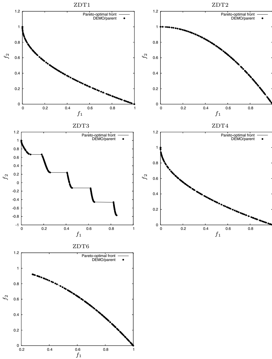
Fig. 4. Nondominated solutions of the final population obtained by DEMO on five ZDT test problems (see Table 7 for more details on these fronts). The presented fronts are the outcome of a single run of DEMO/parent
