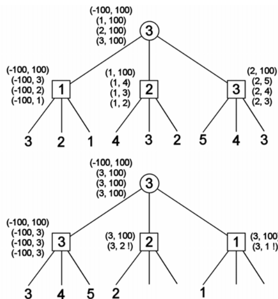
Figure 2. Move ordering
