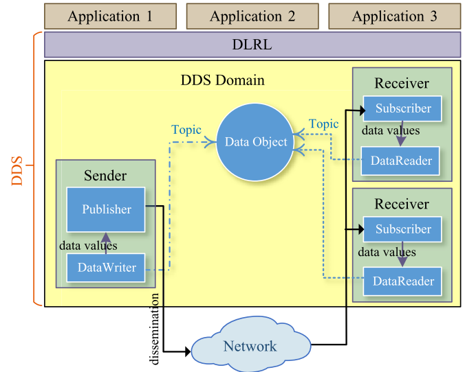
Fig. 16. The conceptual model of DDS.
