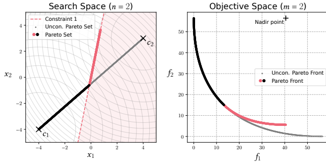
Figure 2: Example problem with two variables, two spherical objectives and a single linear constraint.
